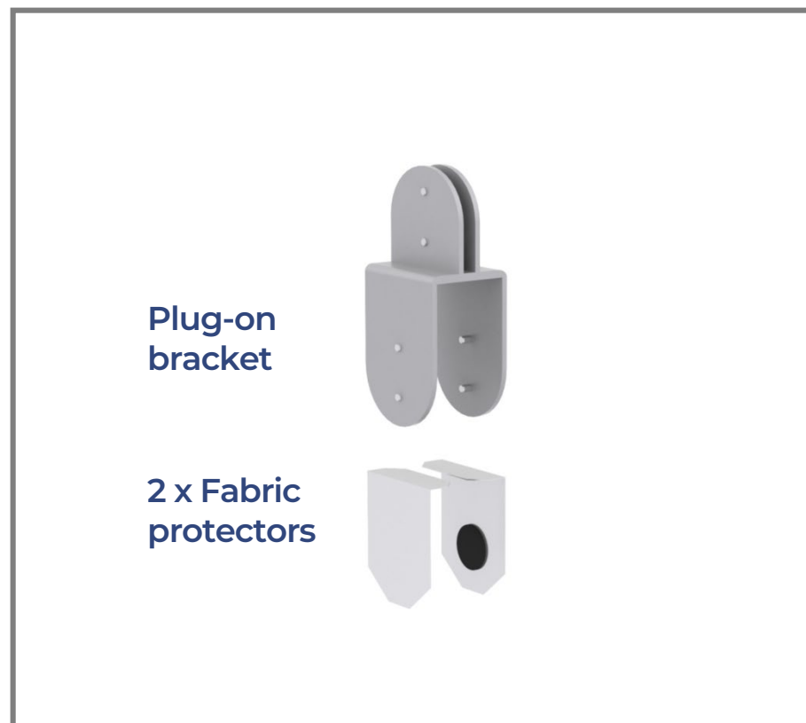
1 Plug-on bracket components
